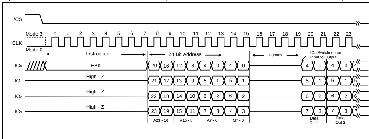
Figure 21a. Fast Read Quad I/O Instruction (Initial instruction or previous M5-4 ≠ 10, SPI Mode)
